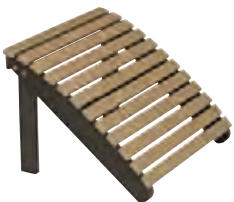
ADIRONDACK FOOTSTOOL | PAFS2400 | 23.5" W X 21" D X 16.5" H
