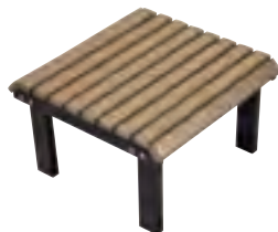
STATIONARY FOOTSTOOL | PVSF2100 | 18.5" W X 19" D X 11" H
